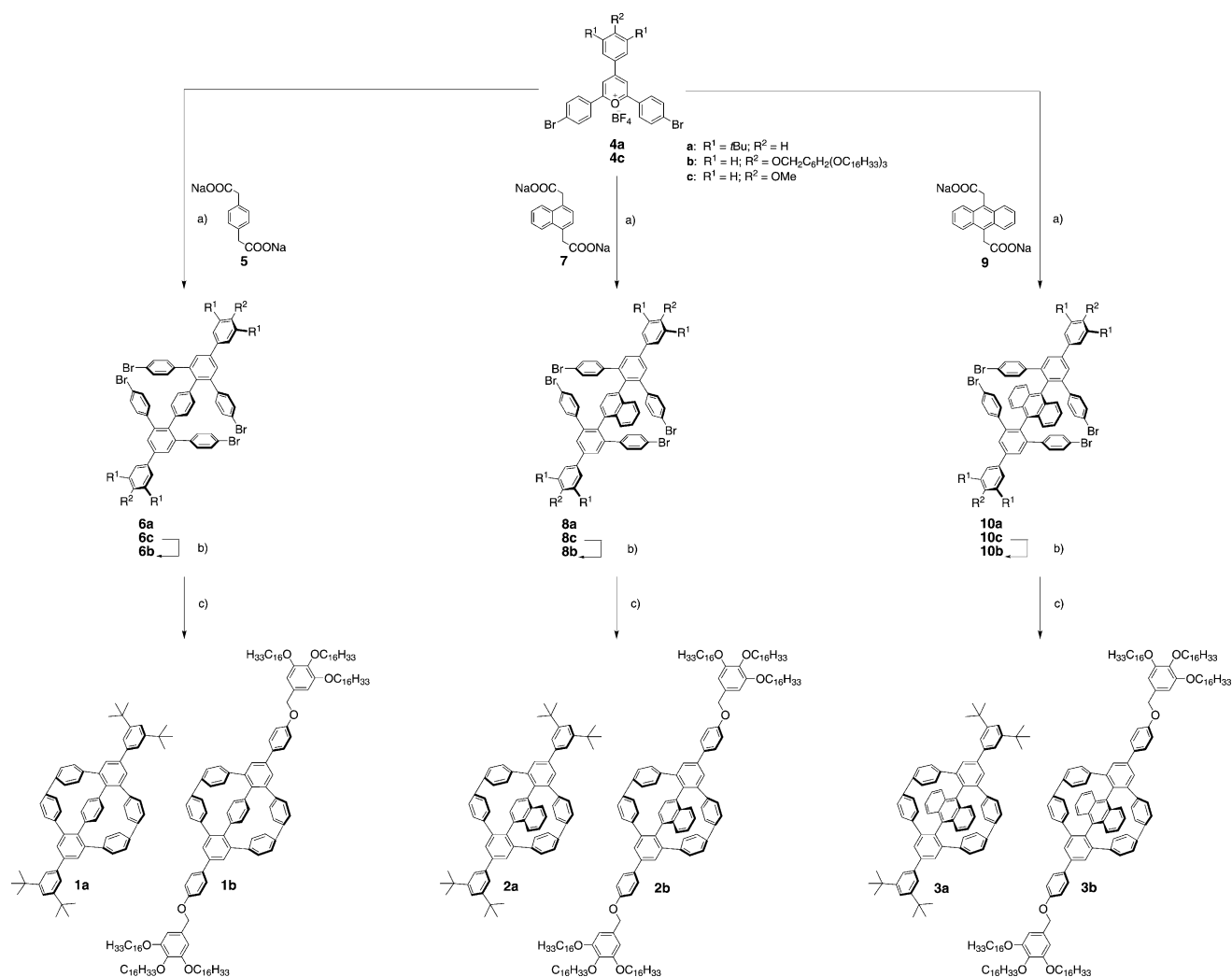
Scheme 1. a) Benzoic anhydride, 150 °C, 3 h; b) 1. BBr_3 , CH_2Cl_2 , -78^\circ C \rightarrow RT , 16 h; 2. 3,4,5-trihexadecyloxybenzyl chloride, Cs_2CO_3 , DMF, 110 °C, 48 h; c) [Ni(cod)_2] , 2,2'-bipyridine, THF/COD, microwave irradiation, 120 °C, 12 min. DMF = N,N -dimethylformamide.
